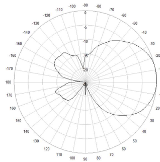
Vertical beamwidth
